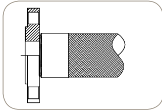
8K - Raised Face, 150lb Fixed Slip-on Flange
